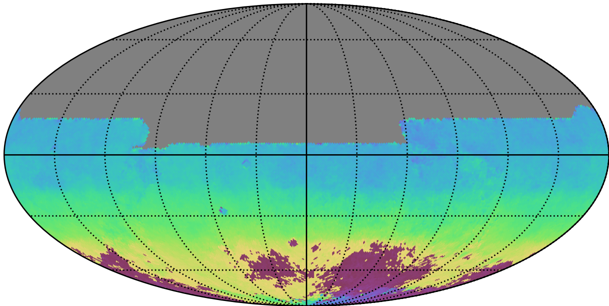
early_u_fpextra3.0_v3.4_10yrs All sky y band: AngleMean rotSkyPos
