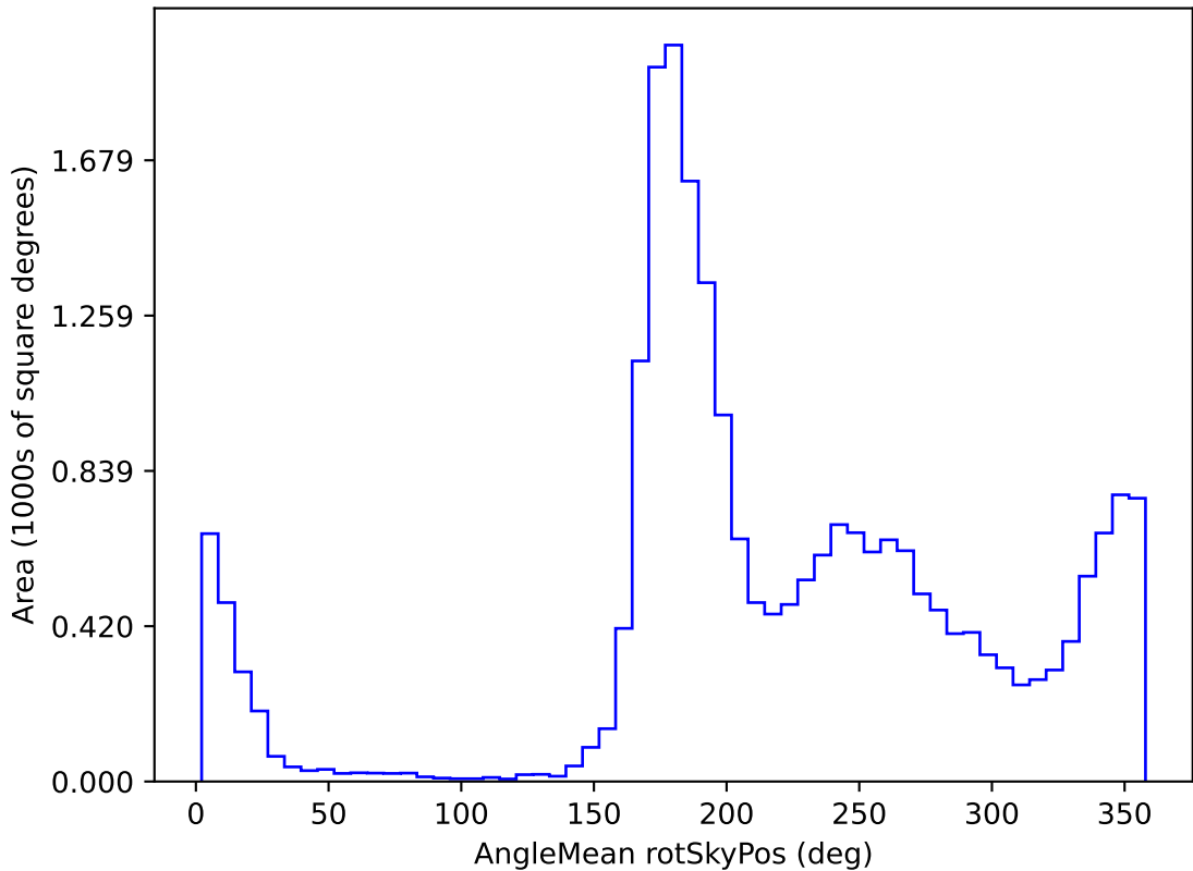
early_u_fpextra3.0_v3.4_10yrs All sky y band: AngleMean rotSkyPos
