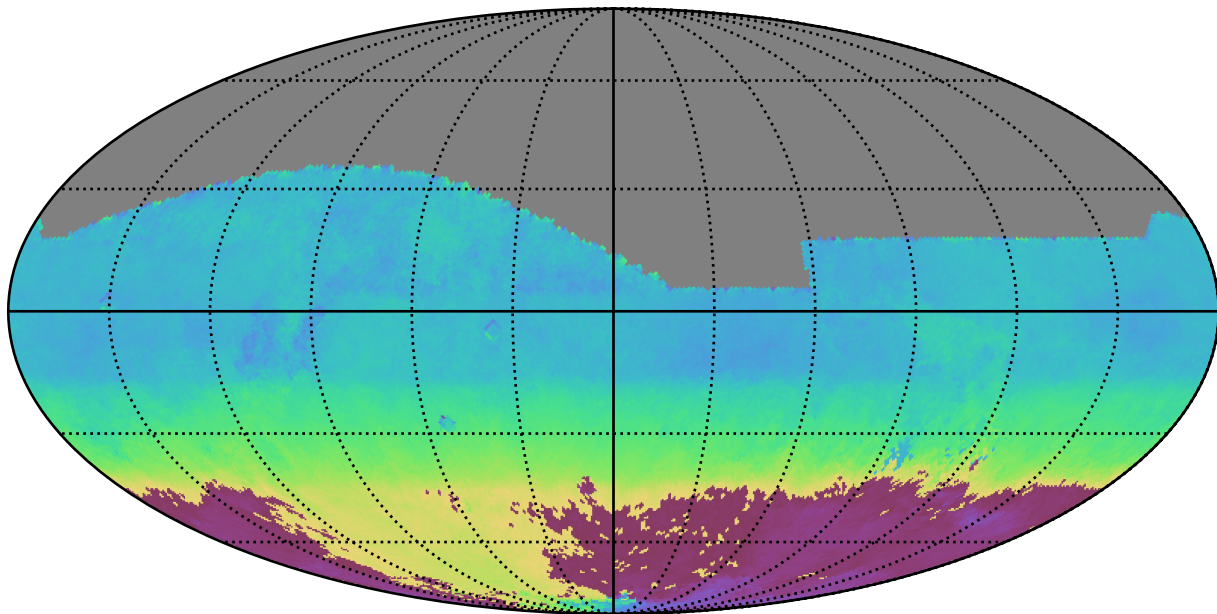
early_u_fpextra3.0_v3.4_10yrs All sky r band: AngleMean rotSkyPos
