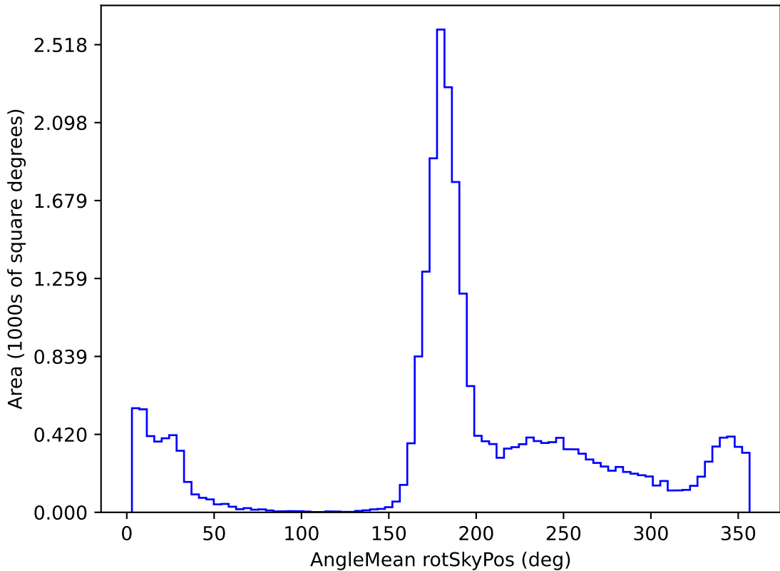
early_u_fpextra3.0_v3.4_10yrs All sky r band: AngleMean rotSkyPos
