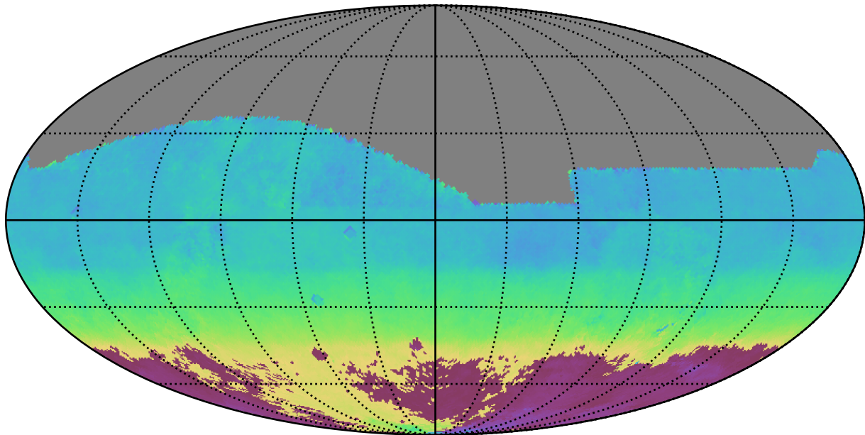
early_u_fpextra3.0_v3.4_10yrs All sky i band: AngleMean rotSkyPos
