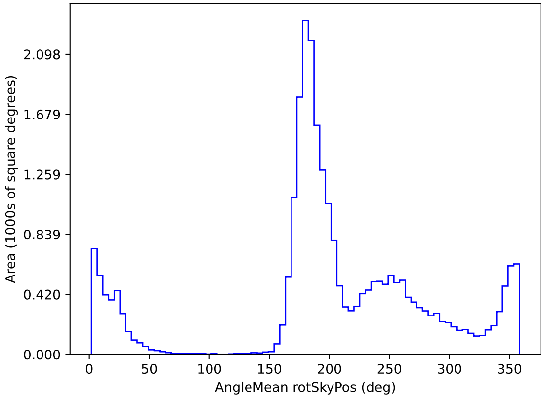
early_u_fpextra3.0_v3.4_10yrs All sky i band: AngleMean rotSkyPos
