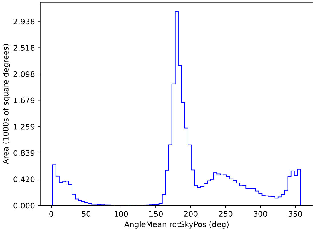
early_u_fpextra3.0_v3.4_10yrs All sky all bands: AngleMean rotSkyPos
