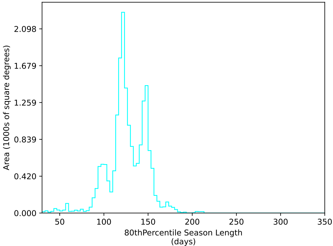
early_u_fpextra3.0_v3.4_10yrs WFD u band: 80thPercentile Season Length
