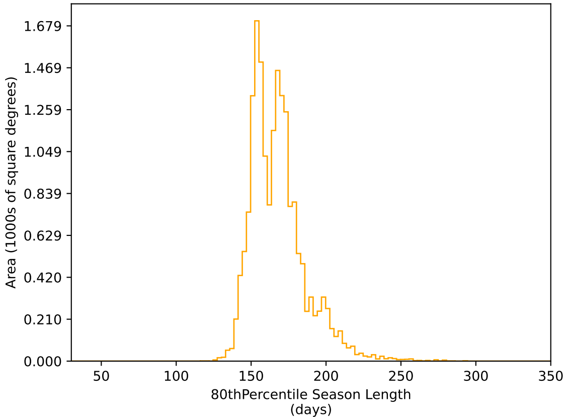
early_u_fpextra3.0_v3.4_10yrs WFD r band: 80thPercentile Season Length
