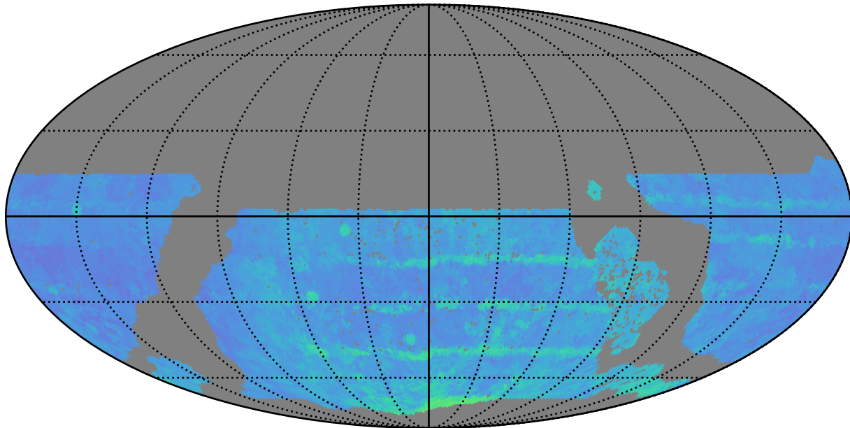
early_u_fpextra3.0_v3.4_10yrs WFD i band: 80thPercentile Season Length
