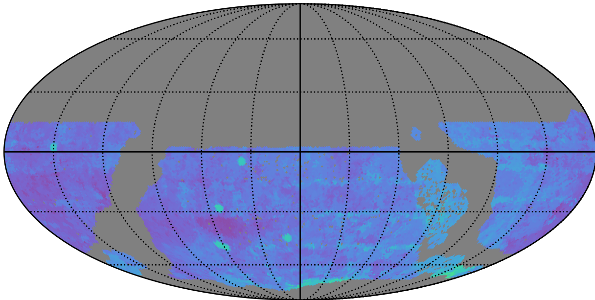
early_u_fpextra3.0_v3.4_10yrs WFD g band: 80thPercentile Season Length
