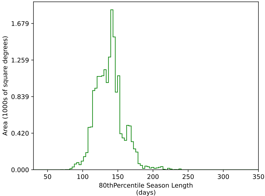
early_u_fpextra3.0_v3.4_10yrs WFD g band: 80thPercentile Season Length
