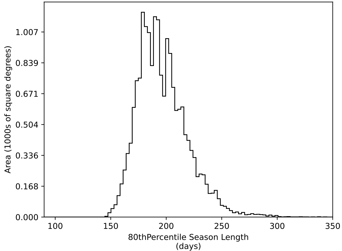
early_u_fpextra3.0_v3.4_10yrs WFD all bands: 80thPercentile Season Length
