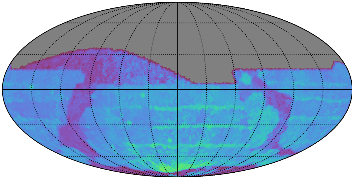
early_u_fpextra3.0_v3.4_10yrs All sky z band: 80thPercentile Season Length
