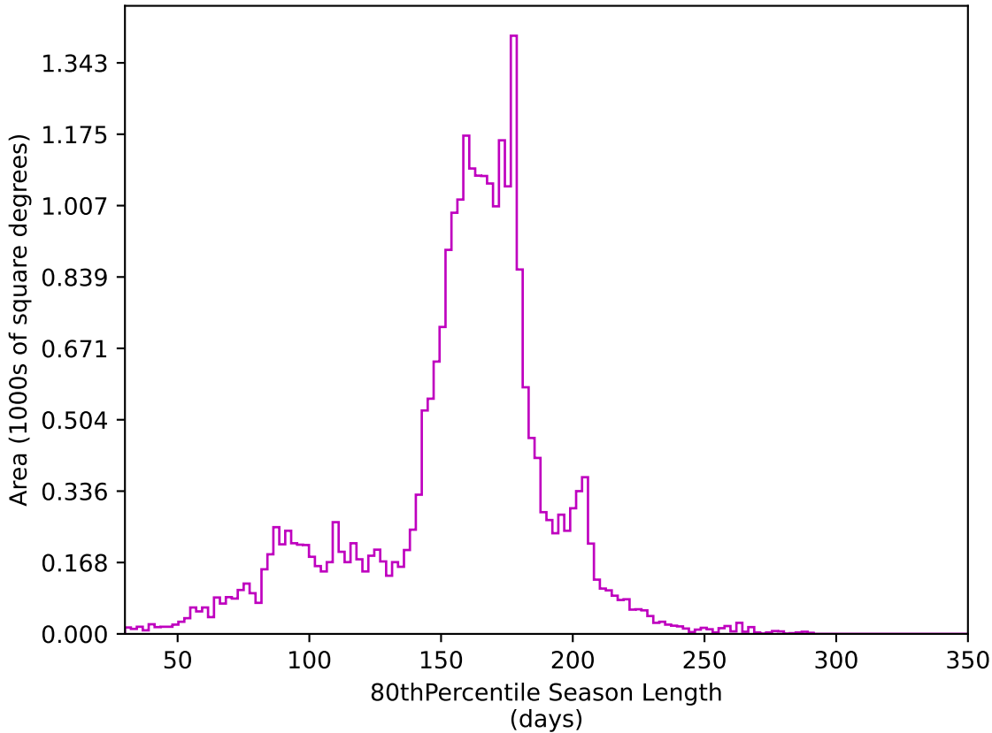
early_u_fpextra3.0_v3.4_10yrs All sky z band: 80thPercentile Season Length
