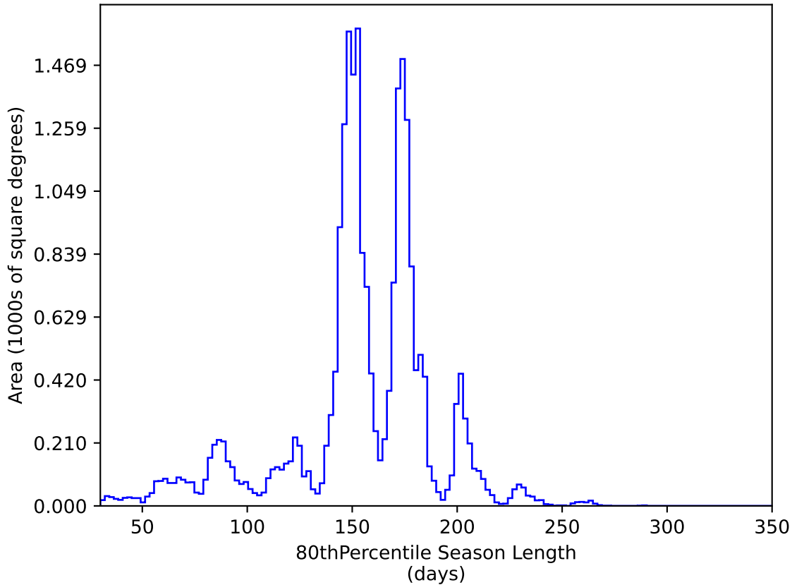
early_u_fpextra3.0_v3.4_10yrs All sky y band: 80thPercentile Season Length
