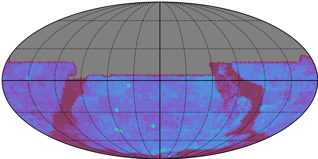
early_u_fpextra3.0_v3.4_10yrs All sky u band: 80thPercentile Season Length
