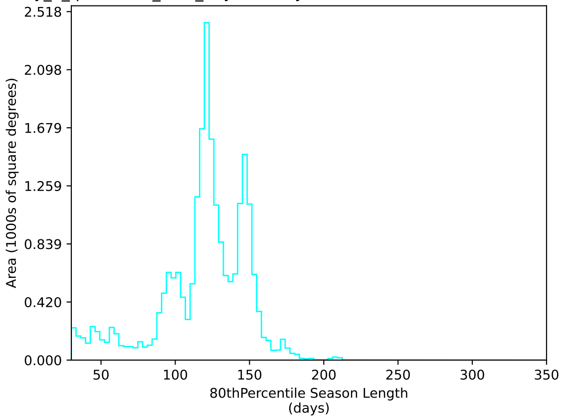
early_u_fpextra3.0_v3.4_10yrs All sky u band: 80thPercentile Season Length
