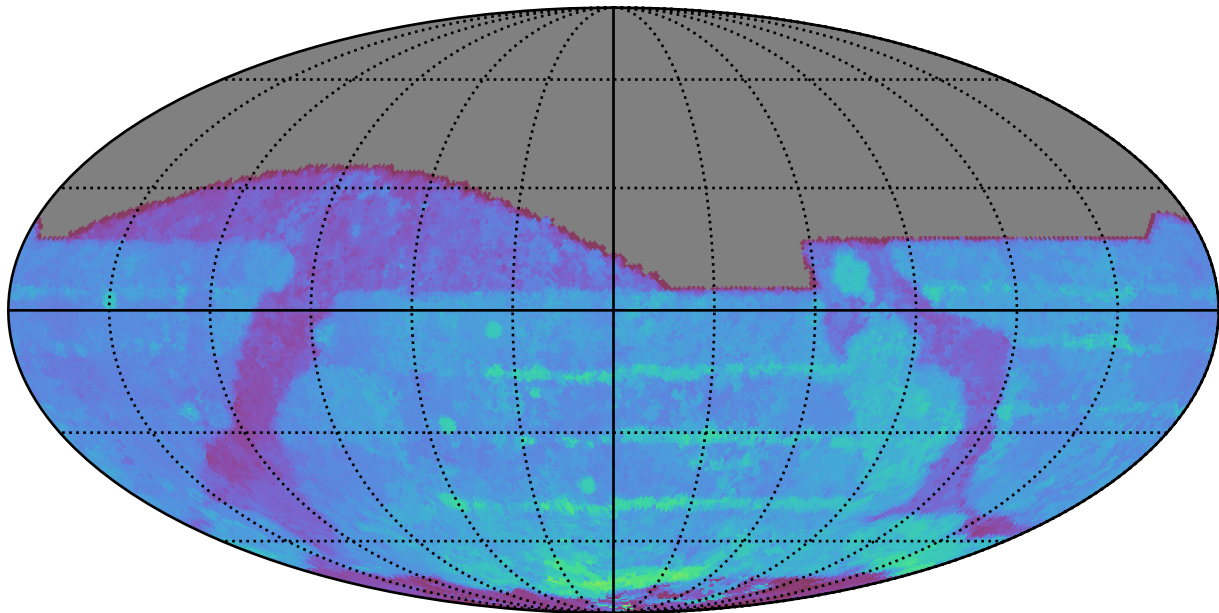
early_u_fpextra3.0_v3.4_10yrs All sky r band: 80thPercentile Season Length
