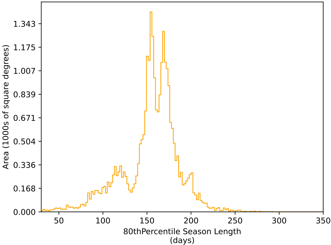
early_u_fpextra3.0_v3.4_10yrs All sky r band: 80thPercentile Season Length
