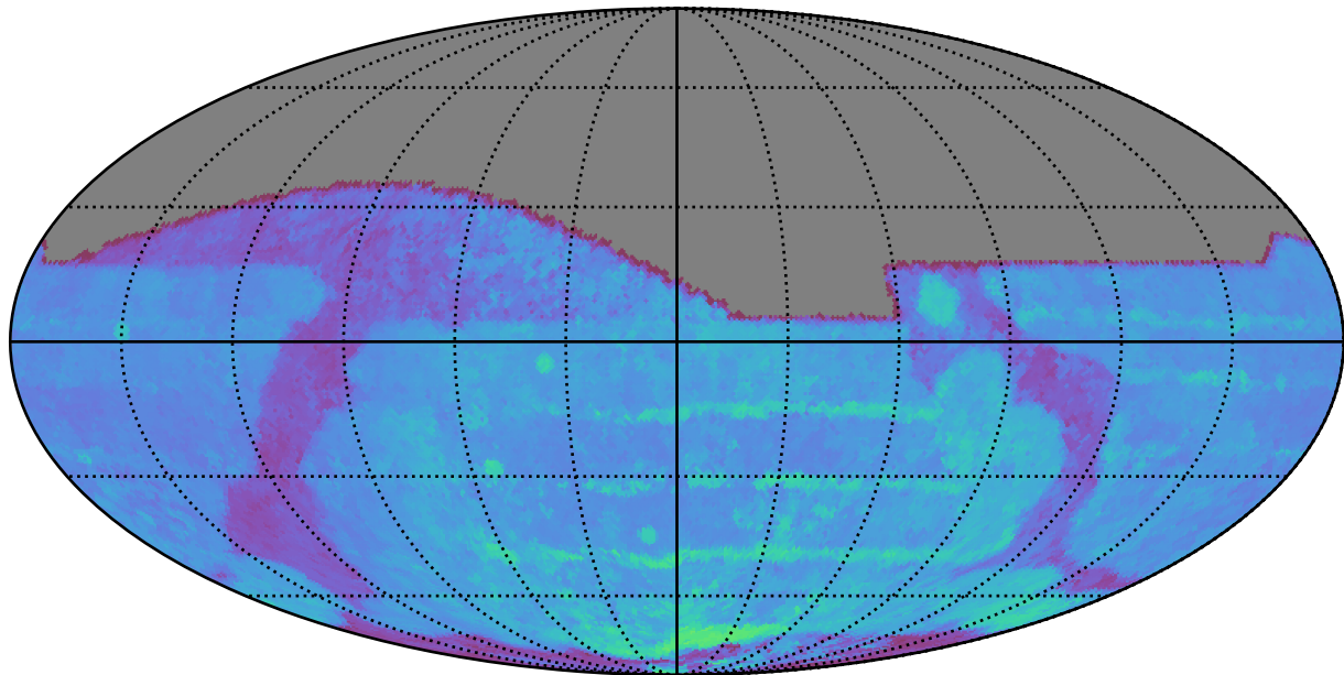
early_u_fpextra3.0_v3.4_10yrs All sky i band: 80thPercentile Season Length
