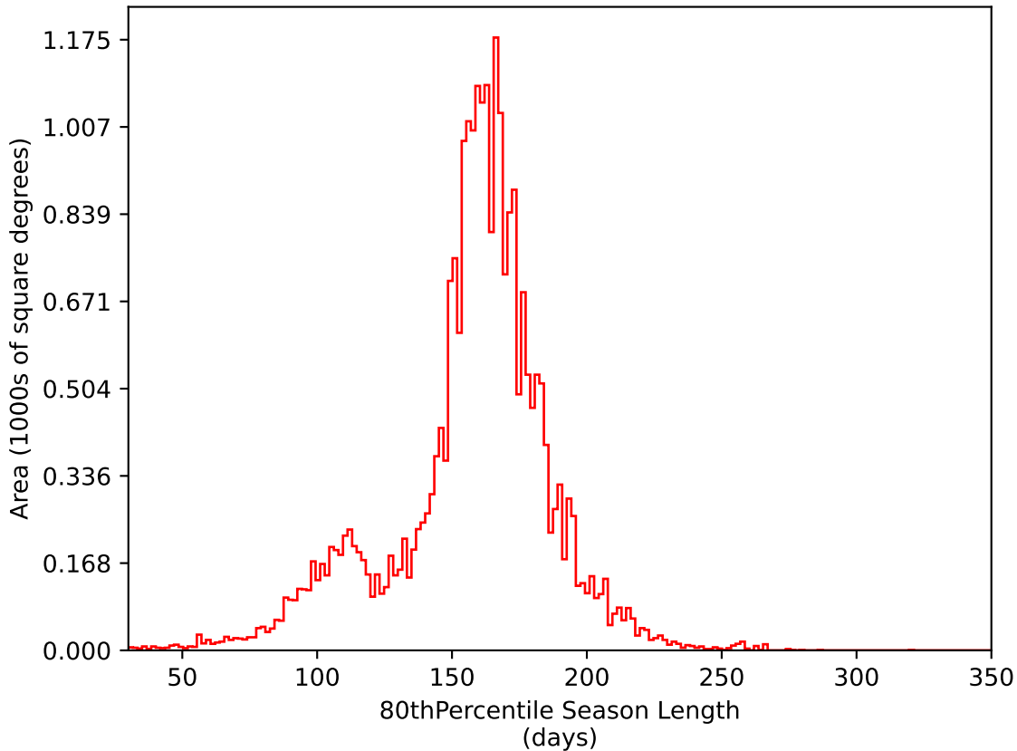
early_u_fpextra3.0_v3.4_10yrs All sky i band: 80thPercentile Season Length
