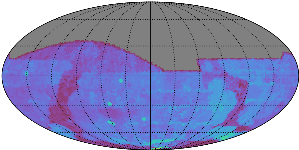
early_u_fpextra3.0_v3.4_10yrs All sky g band: 80thPercentile Season Length
