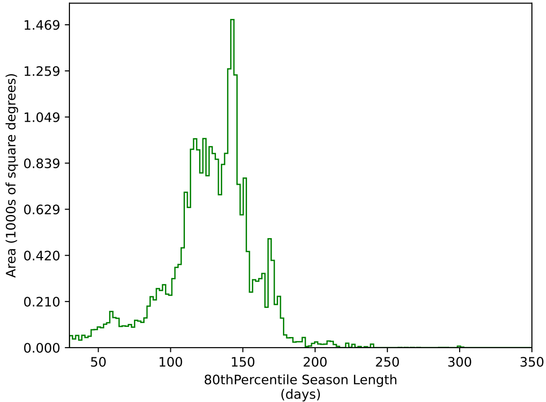
early_u_fpextra3.0_v3.4_10yrs All sky g band: 80thPercentile Season Length
