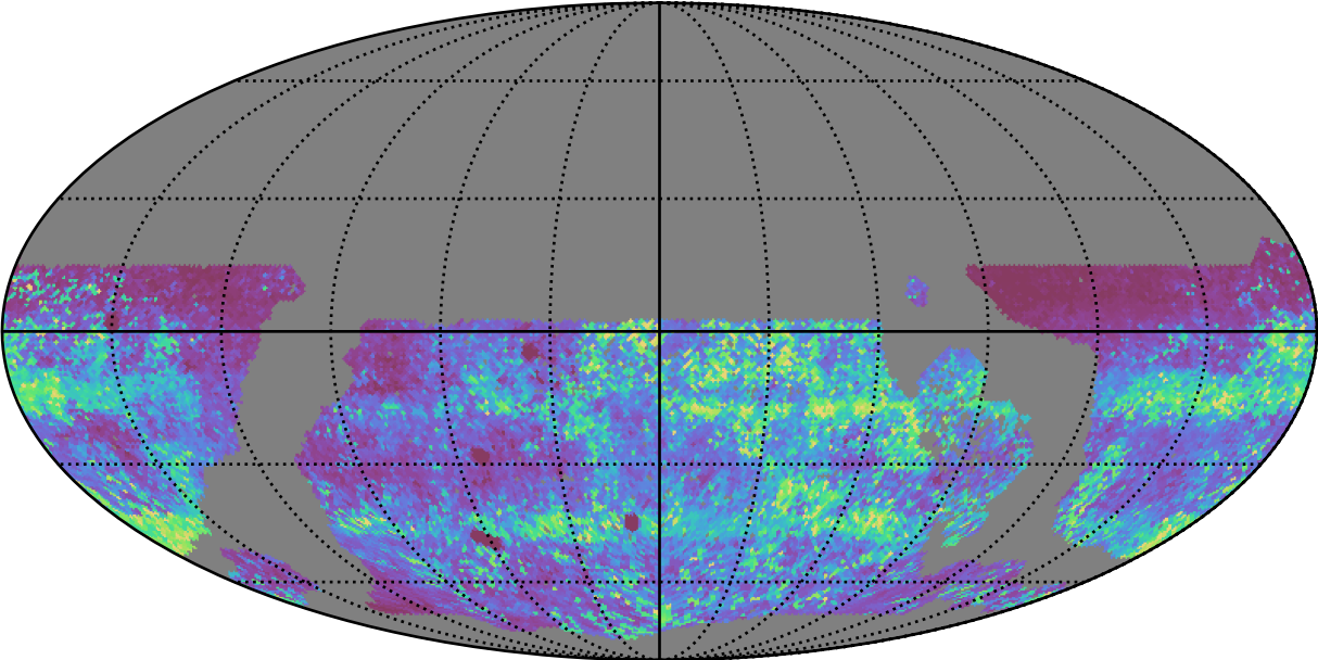
early_u_fpextra3.0_v3.4_10yrs WFD zy bands: 75th Percentile Intranight Timespan
