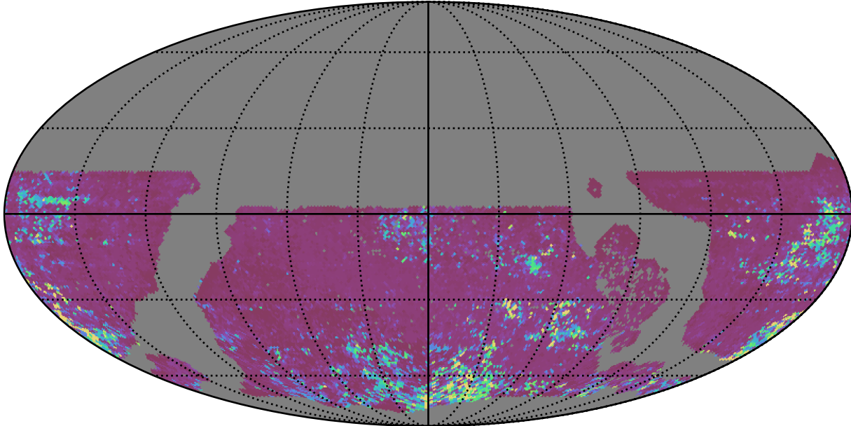
early_u_fpextra3.0_v3.4_10yrs WFD z band: 75th Percentile Intranight Timespan
