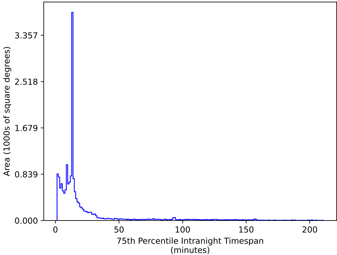
early_u_fpextra3.0_v3.4_10yrs WFD z band: 75th Percentile Intranight Timespan
