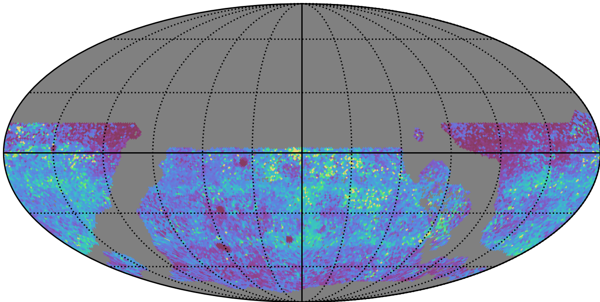
early_u_fpextra3.0_v3.4_10yrs WFD y band: 75th Percentile Intranight Timespan
