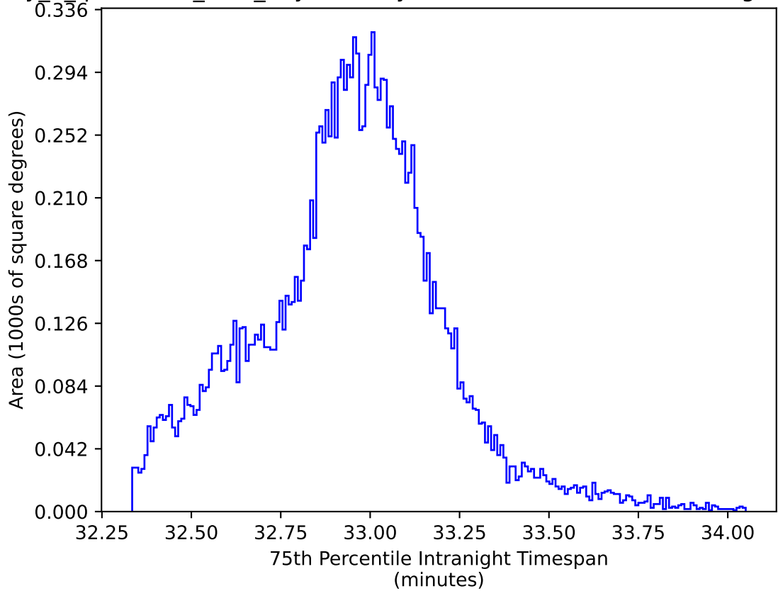
early_u_fpextra3.0_v3.4_10yrs WFD y band: 75th Percentile Intranight Timespan
