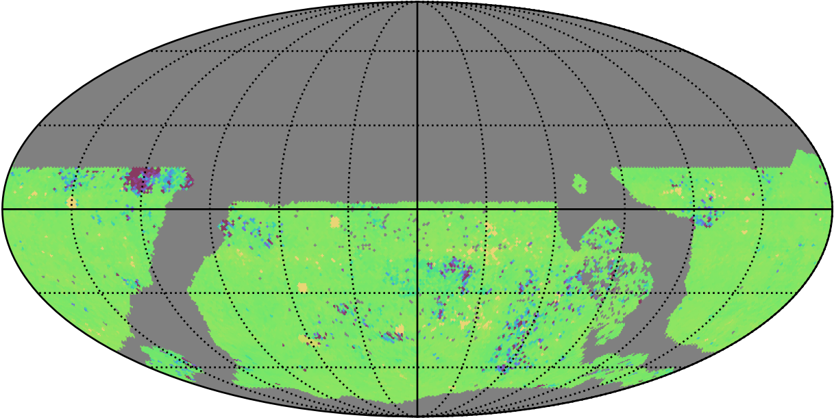
early_u_fpextra3.0_v3.4_10yrs WFD ug bands: 75th Percentile Intranight Timespan
