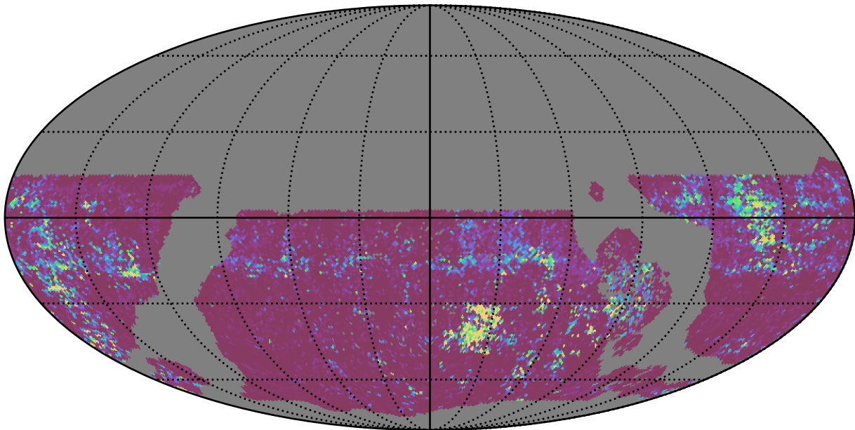
early_u_fpextra3.0_v3.4_10yrs WFD u band: 75th Percentile Intranight Timespan
