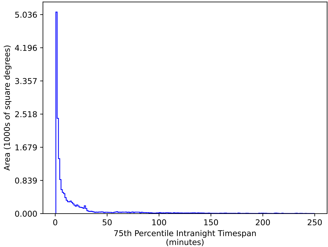
early_u_fpextra3.0_v3.4_10yrs WFD u band: 75th Percentile Intranight Timespan
