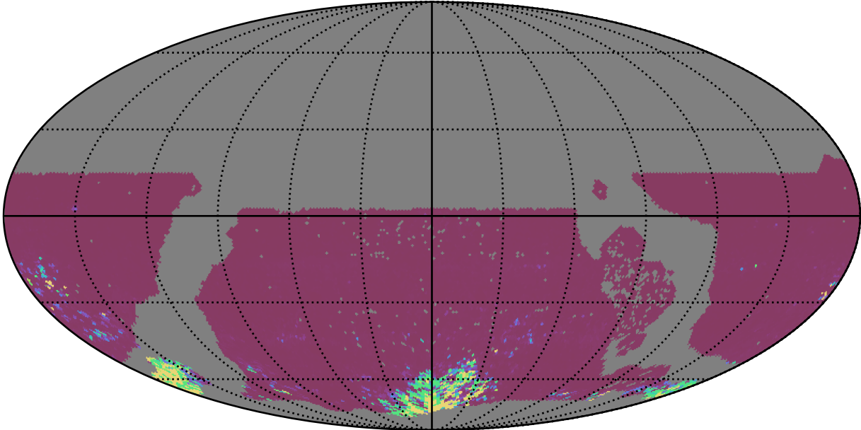
early_u_fpextra3.0_v3.4_10yrs WFD ri bands: 75th Percentile Intranight Timespan
