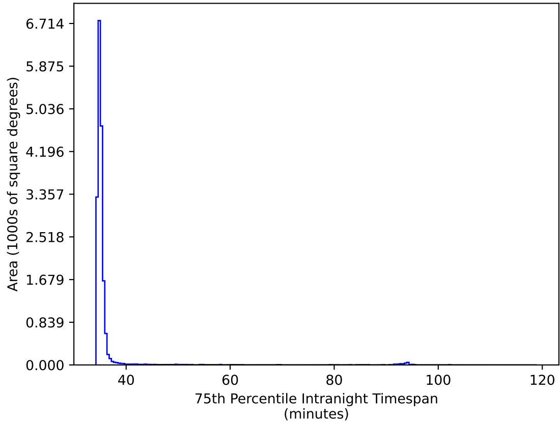
early_u_fpextra3.0_v3.4_10yrs WFD ri bands: 75th Percentile Intranight Timespan
