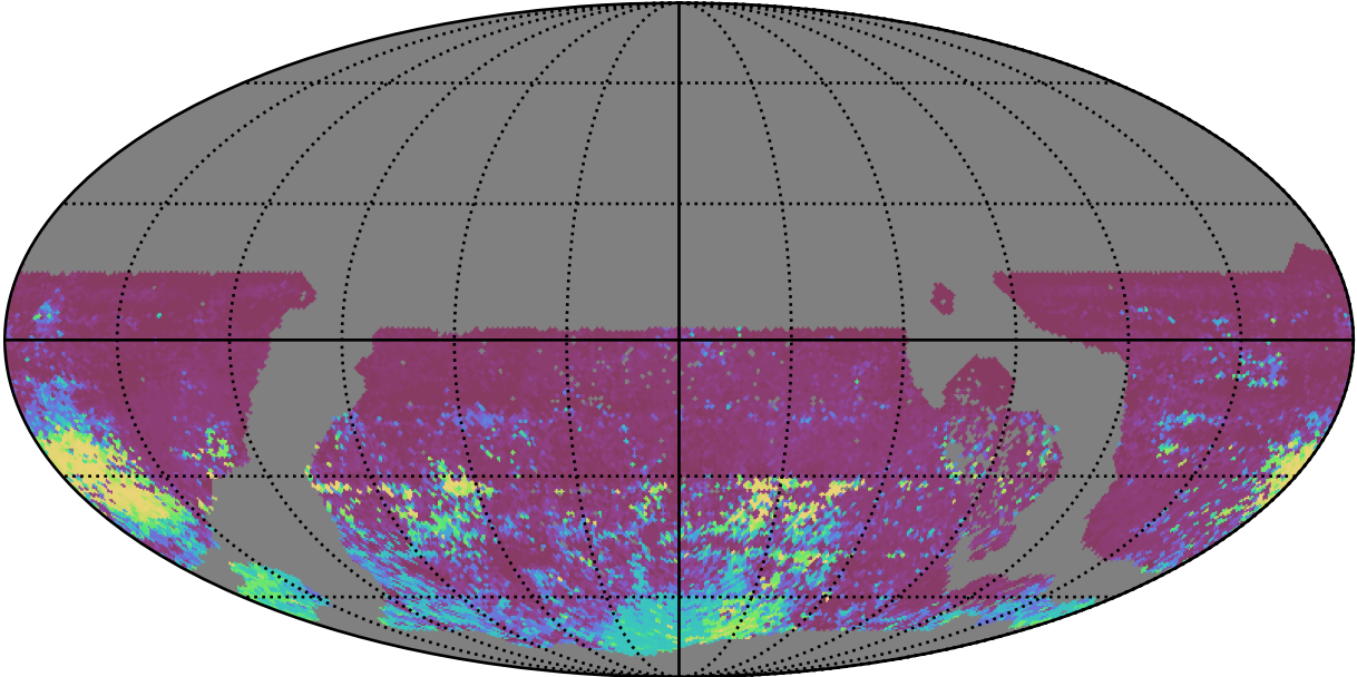
early_u_fpextra3.0_v3.4_10yrs WFD r band: 75th Percentile Intranight Timespan
