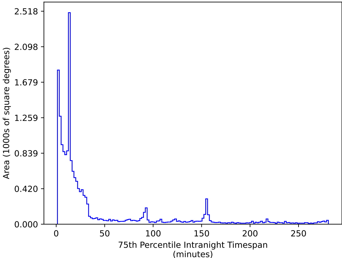
early_u_fpextra3.0_v3.4_10yrs WFD r band: 75th Percentile Intranight Timespan
