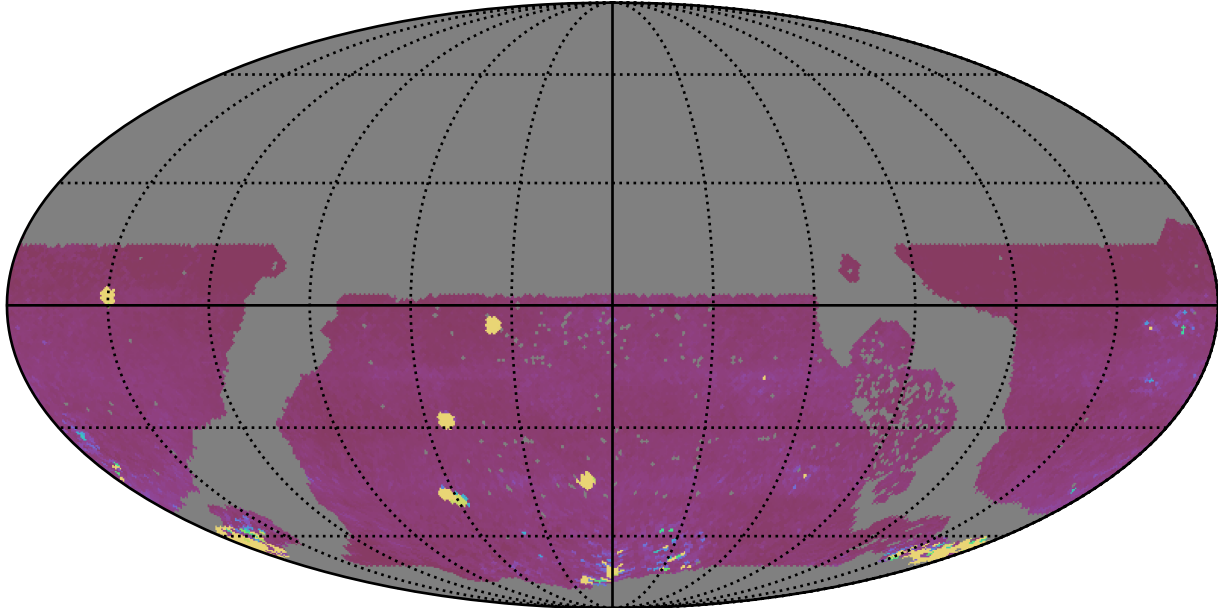
early_u_fpextra3.0_v3.4_10yrs WFD iz bands: 75th Percentile Intranight Timespan
