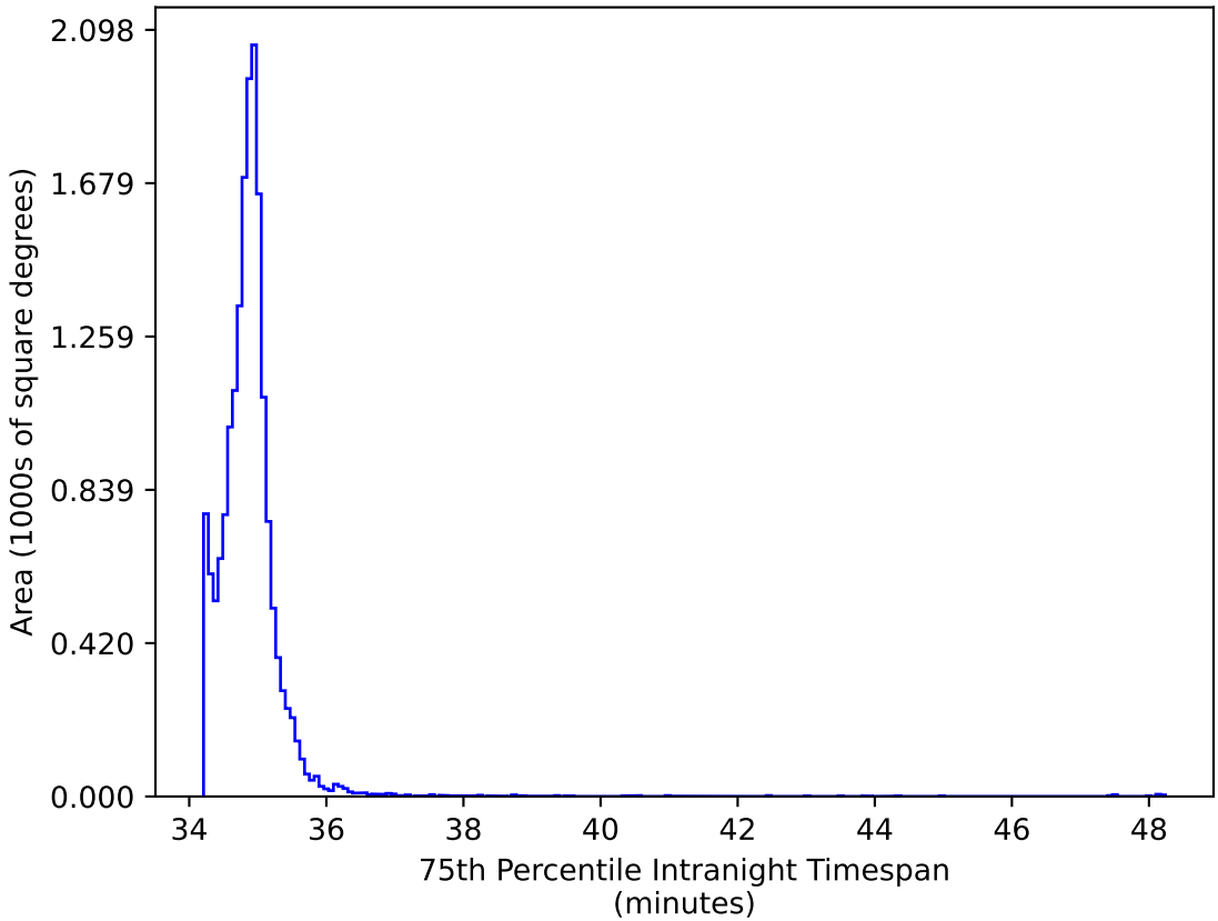
early_u_fpextra3.0_v3.4_10yrs WFD iz bands: 75th Percentile Intranight Timespan
