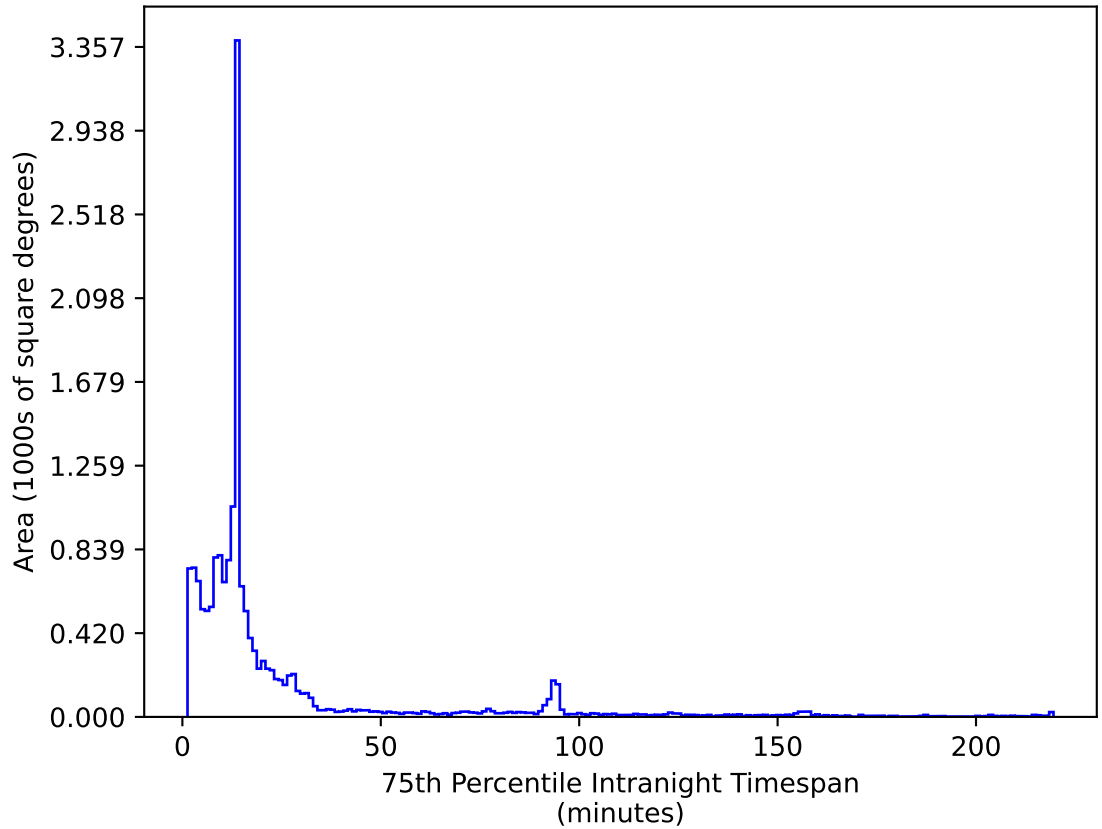
early_u_fpextra3.0_v3.4_10yrs WFD i band: 75th Percentile Intranight Timespan
