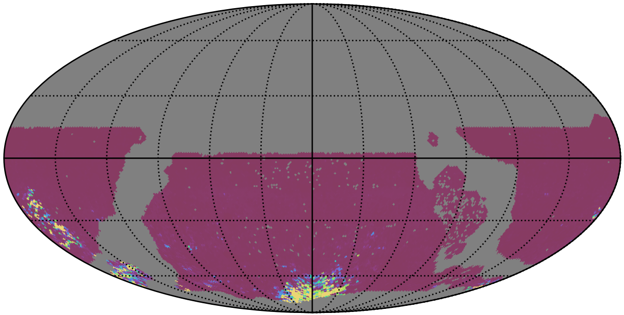
early_u_fpextra3.0_v3.4_10yrs WFD gr bands: 75th Percentile Intranight Timespan
