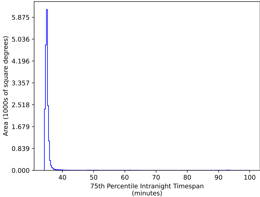
early_u_fpextra3.0_v3.4_10yrs WFD gr bands: 75th Percentile Intranight Timespan
