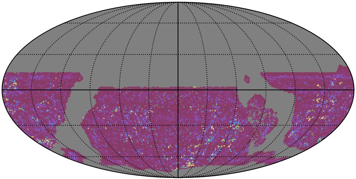
early_u_fpextra3.0_v3.4_10yrs WFD g band: 75th Percentile Intranight Timespan
