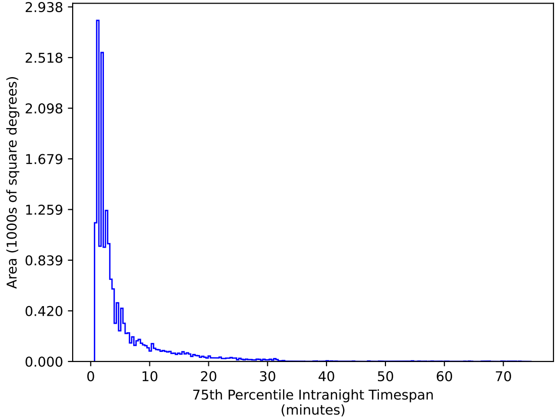
early_u_fpextra3.0_v3.4_10yrs WFD g band: 75th Percentile Intranight Timespan
