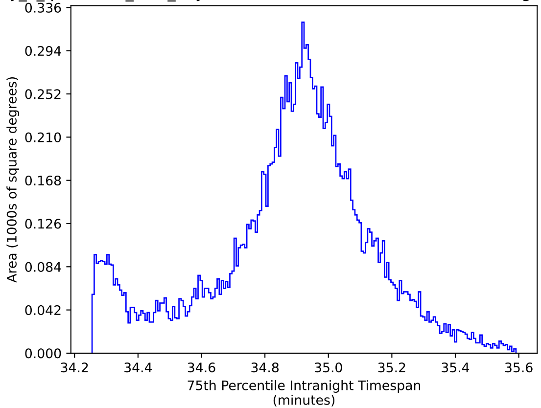
early_u_fpextra3.0_v3.4_10yrs WFD all bands: 75th Percentile Intranight Timespan
