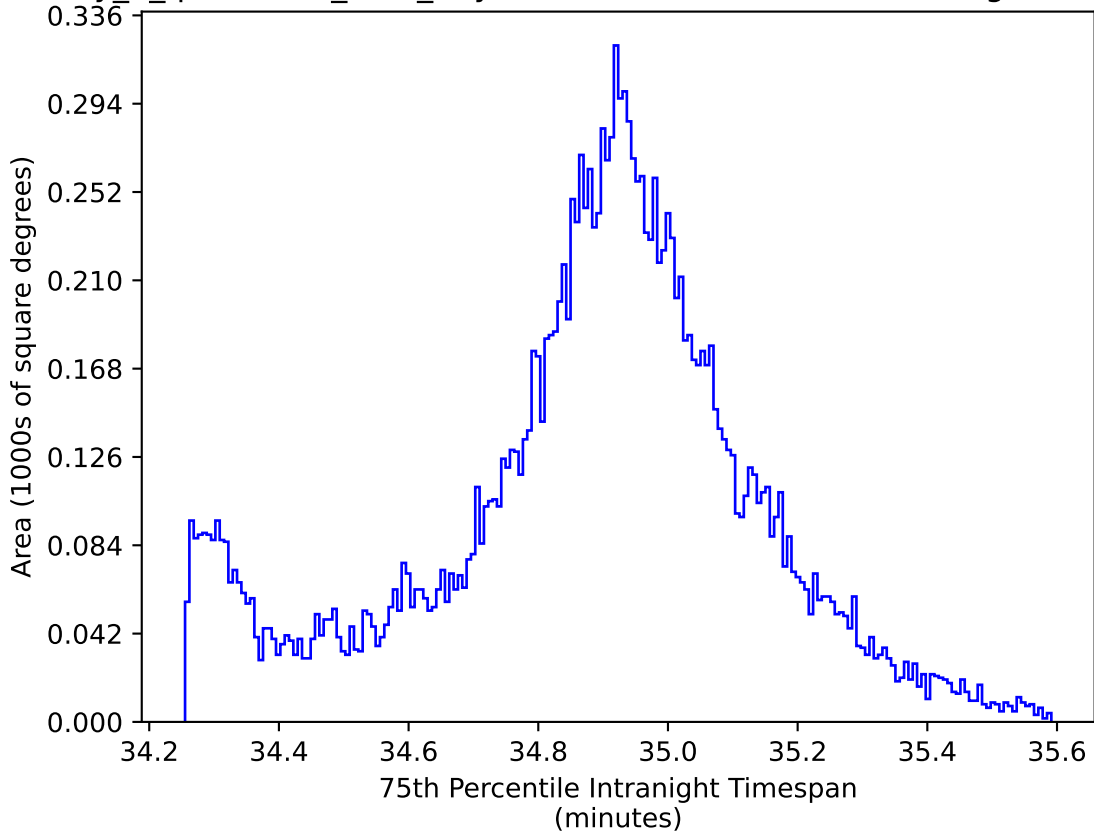
early_u_fpextra3.0_v3.4_10yrs WFD: 75th Percentile Intranight Timespan
