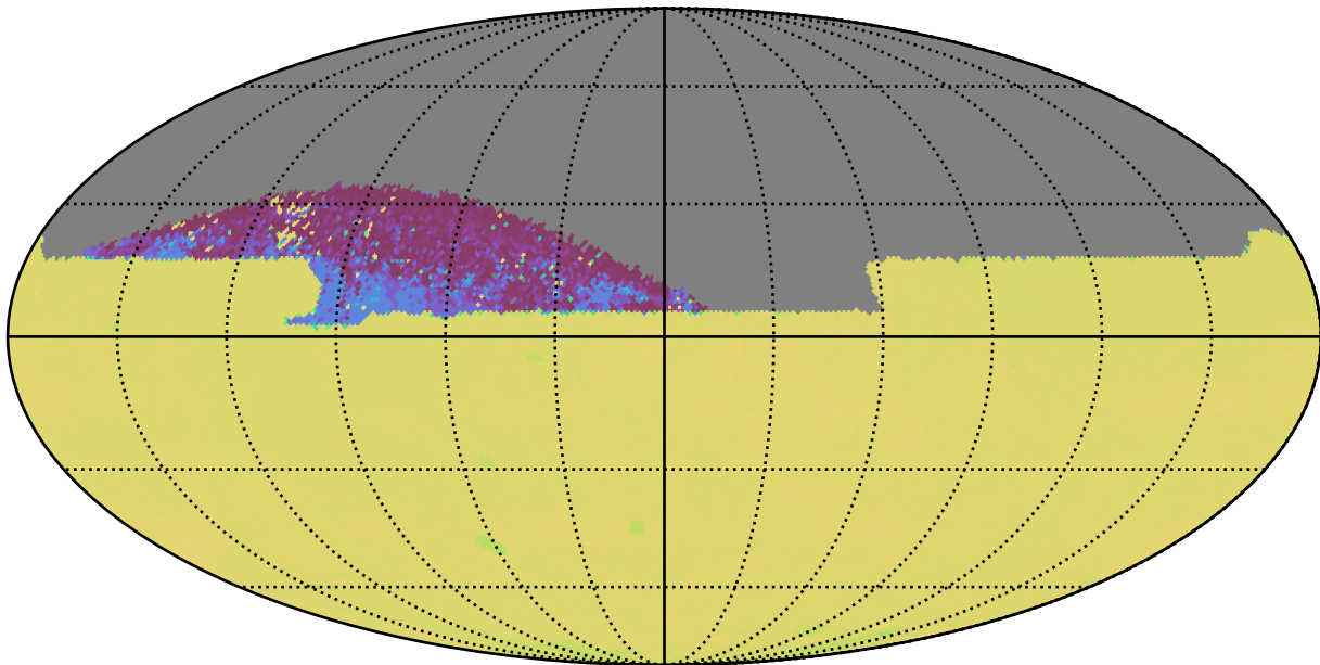
early_u_fpextra3.0_v3.4_10yrs All sky zy bands: 75th Percentile Intranight Timespan
