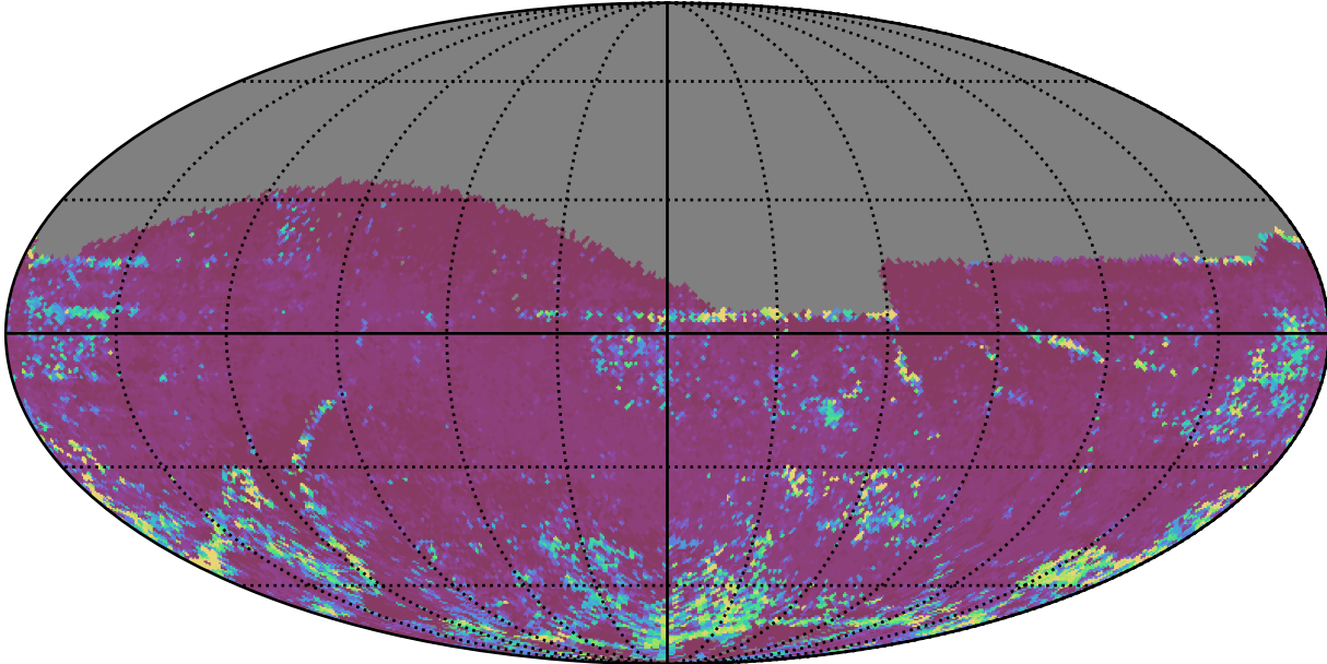
early_u_fpextra3.0_v3.4_10yrs All sky z band: 75th Percentile Intranight Timespan
