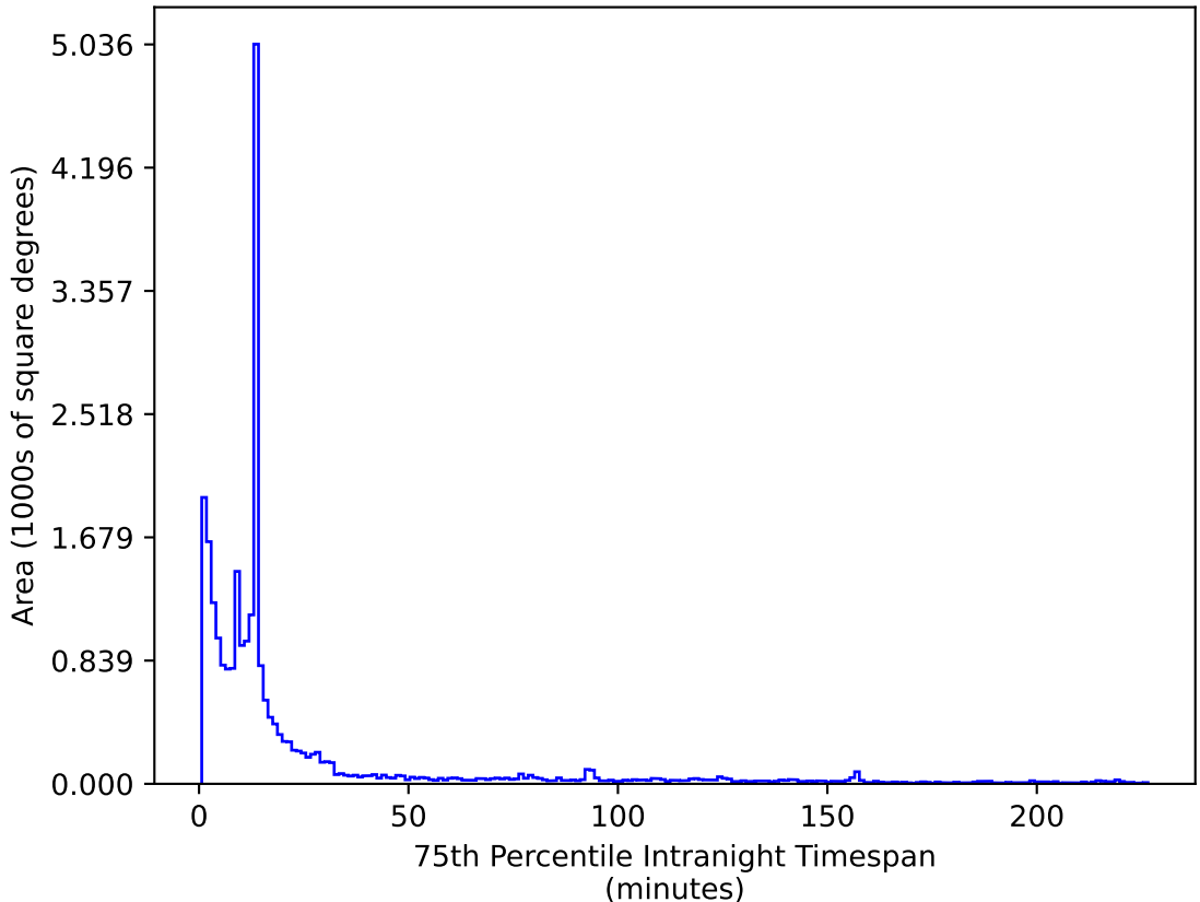
early_u_fpextra3.0_v3.4_10yrs All sky z band: 75th Percentile Intranight Timespan
