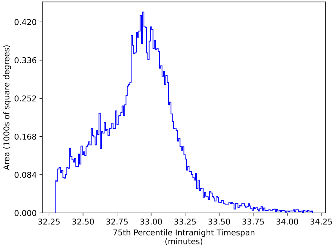
early_u_fpextra3.0_v3.4_10yrs All sky y band: 75th Percentile Intranight Timespan
