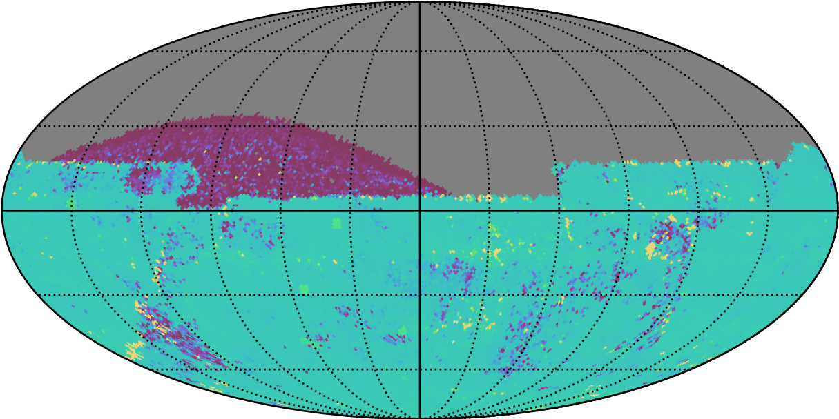
early_u_fpextra3.0_v3.4_10yrs All sky ug bands: 75th Percentile Intranight Timespan
